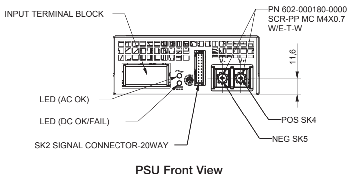
Signal Output Signal Connectors (SK2) SK2 Mating Connector: JST Part Number PHDR-20VS; Contact Pins: JST Part Number SPHD-001T-P0.5
