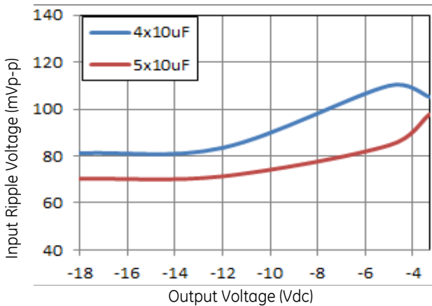
Figure 65. Input ripple voltage with 4x10 \mu F or 5x10 \mu F ceramic capacitors at the input (max load).
