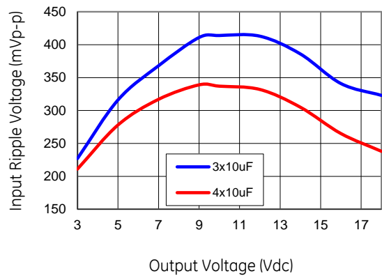
Figure 29. Input ripple voltage for various output voltages with 3 \times 10 \mu F or 4 \times 10 \mu F ceramic capacitors at the input (maximum load). Input voltage is 28V. Scope BW at 20MHz
