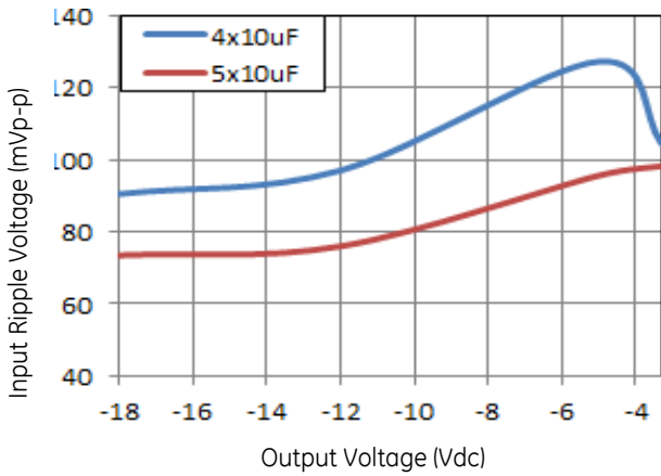
Figure 64. Input ripple voltage with 4x10 \mu F or 5x10 \mu F ceramic capacitors at the input (max load).
