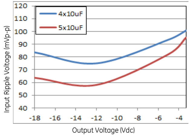
Figure 66. Input ripple voltage with 4x10 \mu F or 5x10 \mu F input ceramic capacitors (max load).
