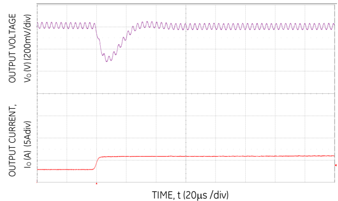
Figure 22. Transient Response to Dynamic Load Change from 50% to 100% at 28Vin, C_{ext} = 5 \times 22\mu F , C_{Tune} = 220pF & R_{Tune} = 200
