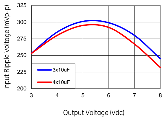
Figure 28. Input ripple voltage for various output voltages with 3 \times 10 \mu F or 4 \times 10 \mu F ceramic capacitors at the input (maximum load). Input voltage is 12V. Scope BW at 20MHz
