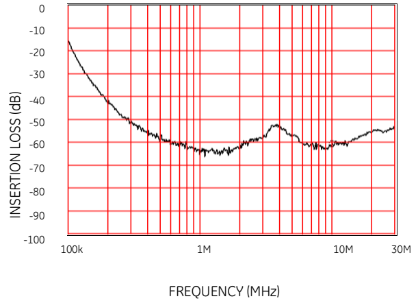
Figure 4: Typical Differential-Mode Insertion Loss in a 50Ω circuit.(-11 Option, 30MHz Axis max.)
