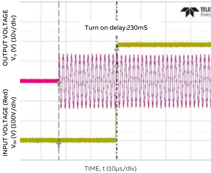
Figure 4. Typical Start-up ( V_{IN} = 90V_{ac} , Full Load)
