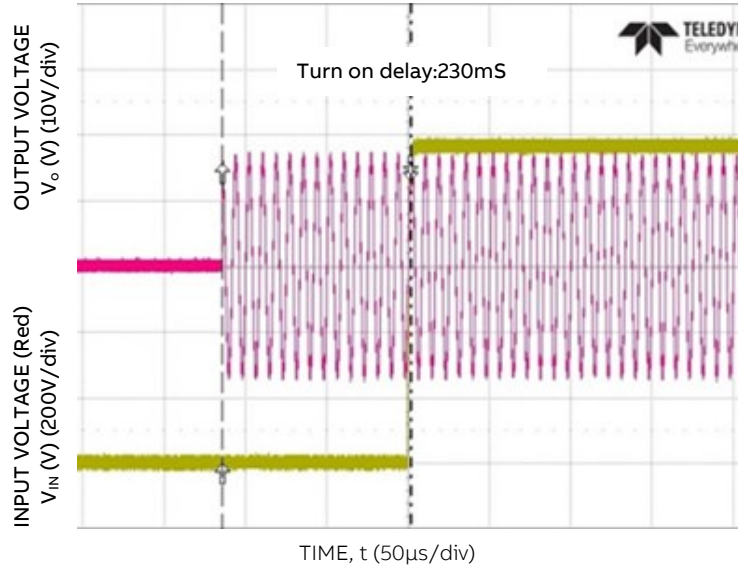
Figure 5. Typical Start-up ( V_{IN} = 230V , Full Load)
