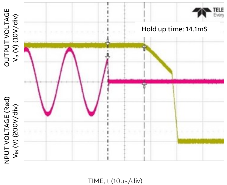
Figure 7. Typical Hold-up Waveforms ( V_{IN} = 230V , 100% Load)
