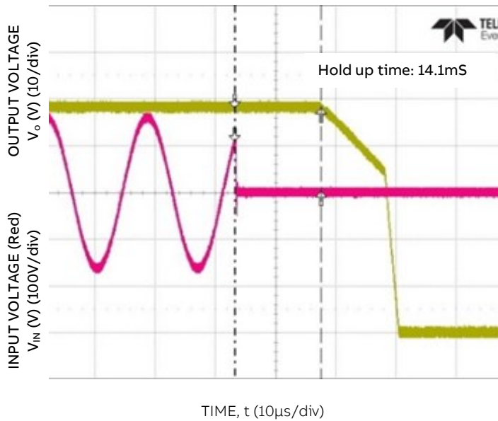
Figure 6. Typical Hold-up Waveforms ( V_{IN} = 115V_{ac} , 100% Load)
