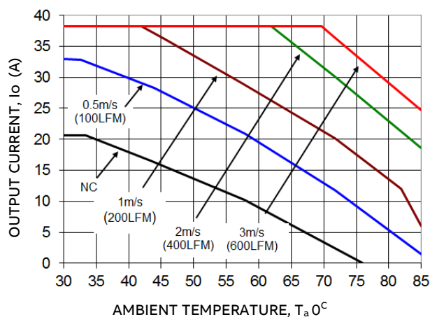
Figure 2: Power. Data shown for model CLP0412FPXXXX03A, 115VAC in. At 230VAC in derating is the same or better. Standby output is loaded at 0.25A. For derating at other input voltages and other models, consult the GE Technical representative.
