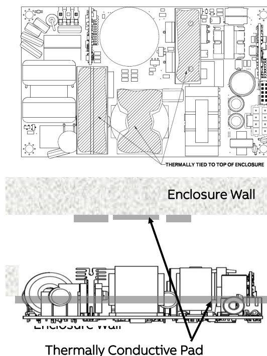
Fig. 11. Example arrangement of the CLP0412 for sealed enclosure applications.
