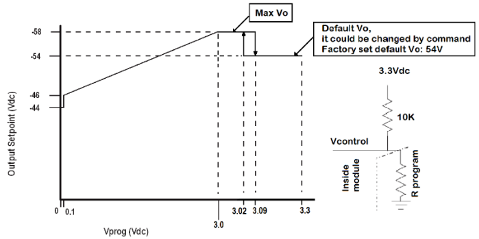
Figure 13. Diagram showing how output can be margined using Vcontrol adjustment.
